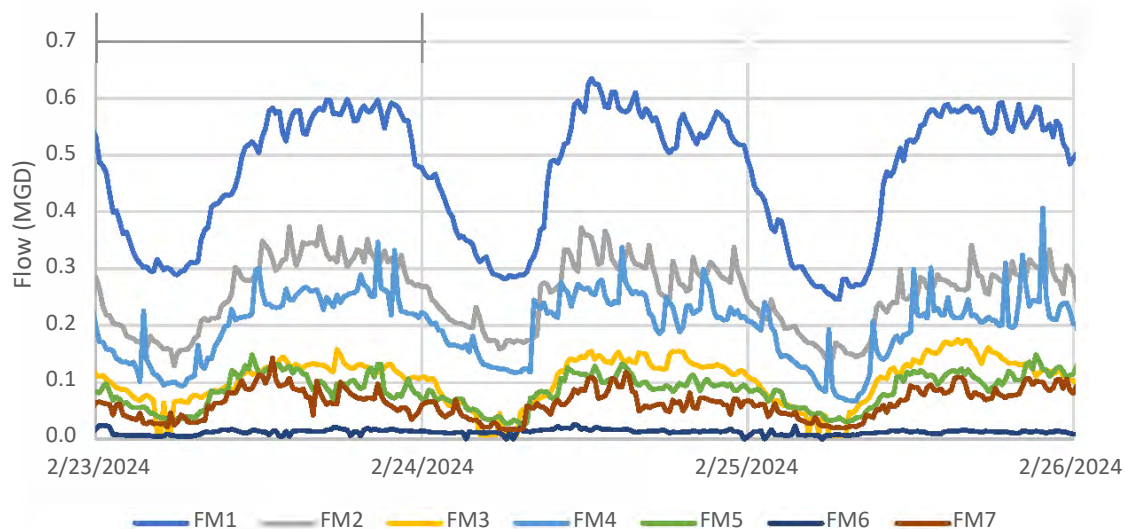
Graph 3 - Turkey Creek Basin Dry-Weather Flow Period 2
