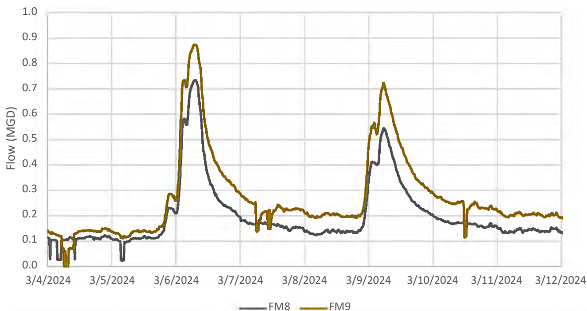
Graph 11 - Dried Indian Creek Basin Flows Rain Event 3
