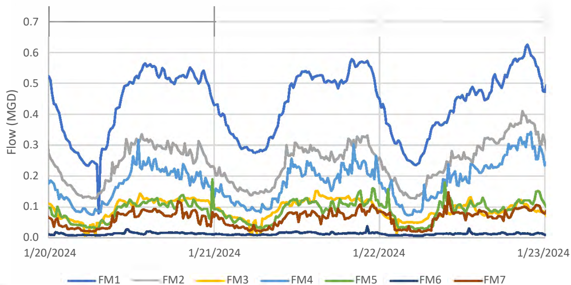
Graph 2 - Turkey Creek Basin Dry-Weather Flow Period 1
