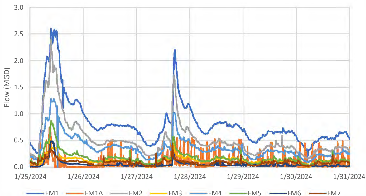
Graph 4 - Turkey Creek Basin Flows Rain Event 1
