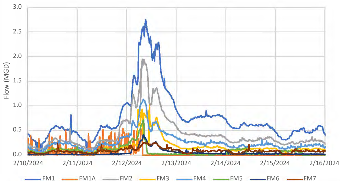
Graph 5 - Turkey Creek Basin Flows Rain Event 2
