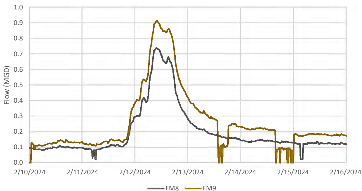
Graph 10 - Dried Indian Creek Basin Flows Rain Event 2
