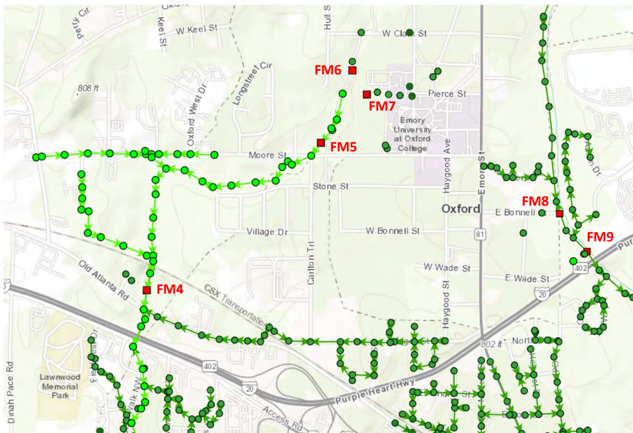
Figure 2 – Turkey Creek (upper end of basin) & Dried Indian Creek Flow Monitor Locations
